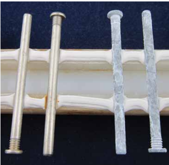
Figure 6: After test, the 305 SST parts remain unchanged (left) while the coated parts (right) exhibit significant white corrosion.
