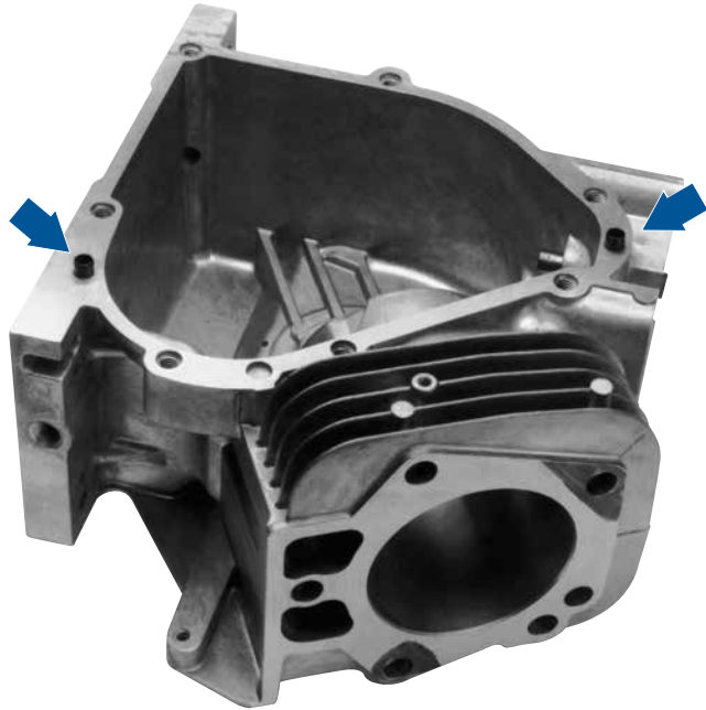
ENGINE HOUSING
