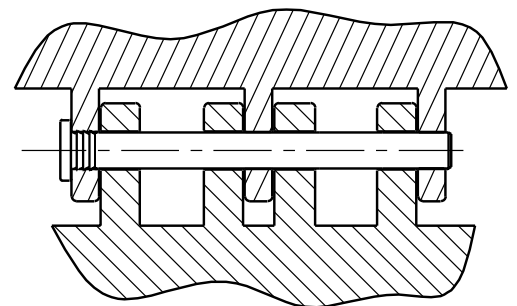
Application example: SPIROL LP500 Latch Pin in Automotive Door Handle
